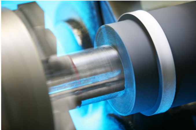
Grinding of rubber covered rollers
